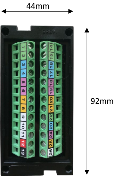
Rear view (Panel cut-out)
