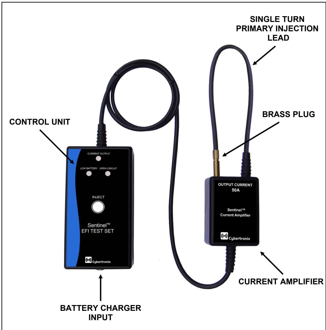
FIGURE 1: Sentinel™ TS-EFI-50
